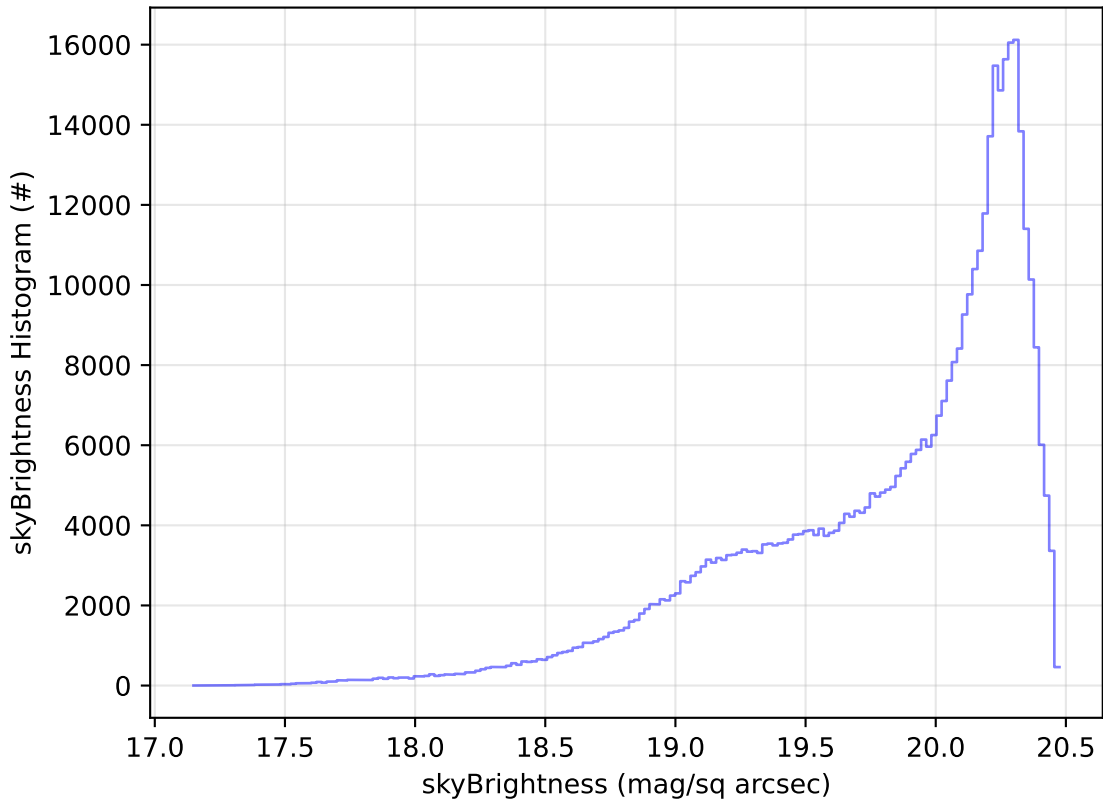
too_combined_s0.5_v3.4_10yrs All sky i band: skyBrightness Histogram
