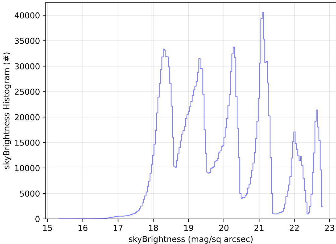
too_combined_s0.5_v3.4_10yrs All sky all bands: skyBrightness Histogram
