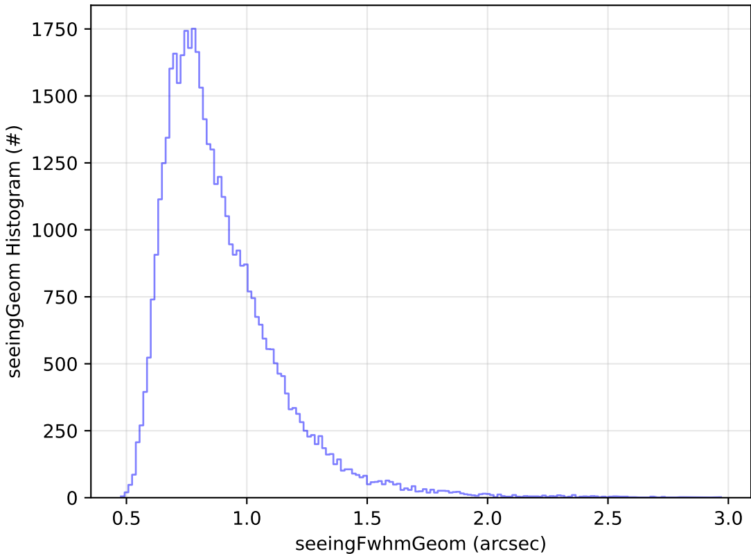
too_combined_s0.5_v3.4_10yrs Yr 1 z band: seeingGeom Histogram
