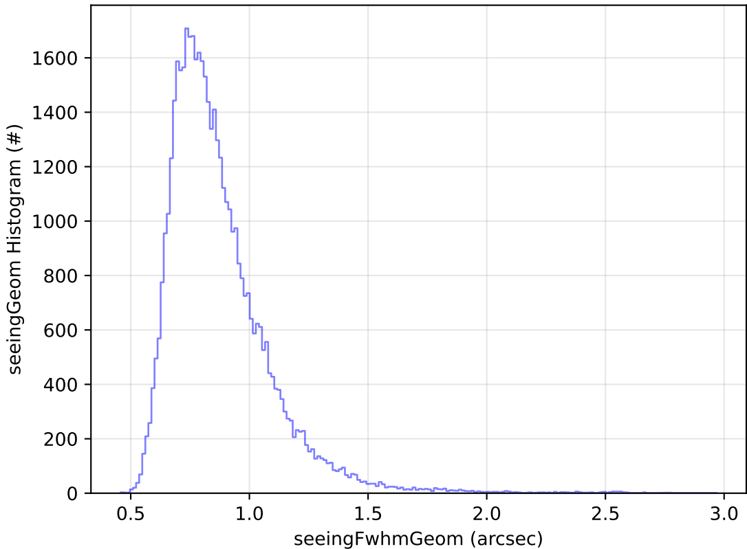
too_combined_s0.5_v3.4_10yrs Yr 1 y band: seeingGeom Histogram
