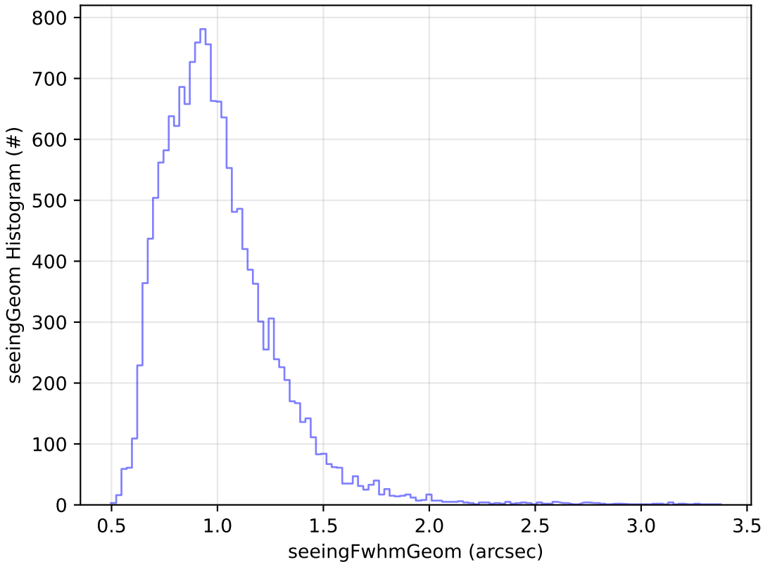
too_combined_s0.5_v3.4_10yrs Yr 1 u band: seeingGeom Histogram
