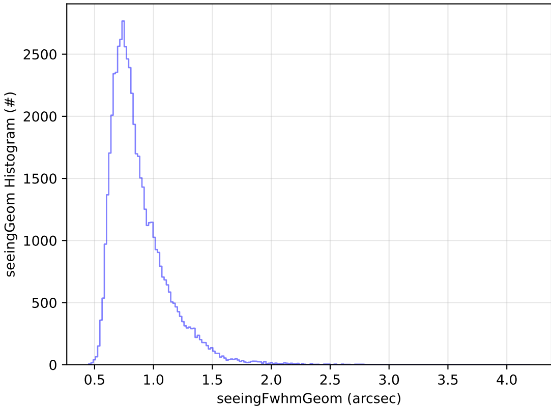
too_combined_s0.5_v3.4_10yrs Yr 1 i band: seeingGeom Histogram
