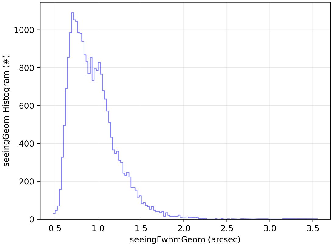
too_combined_s0.5_v3.4_10yrs Yr 1 g band: seeingGeom Histogram
