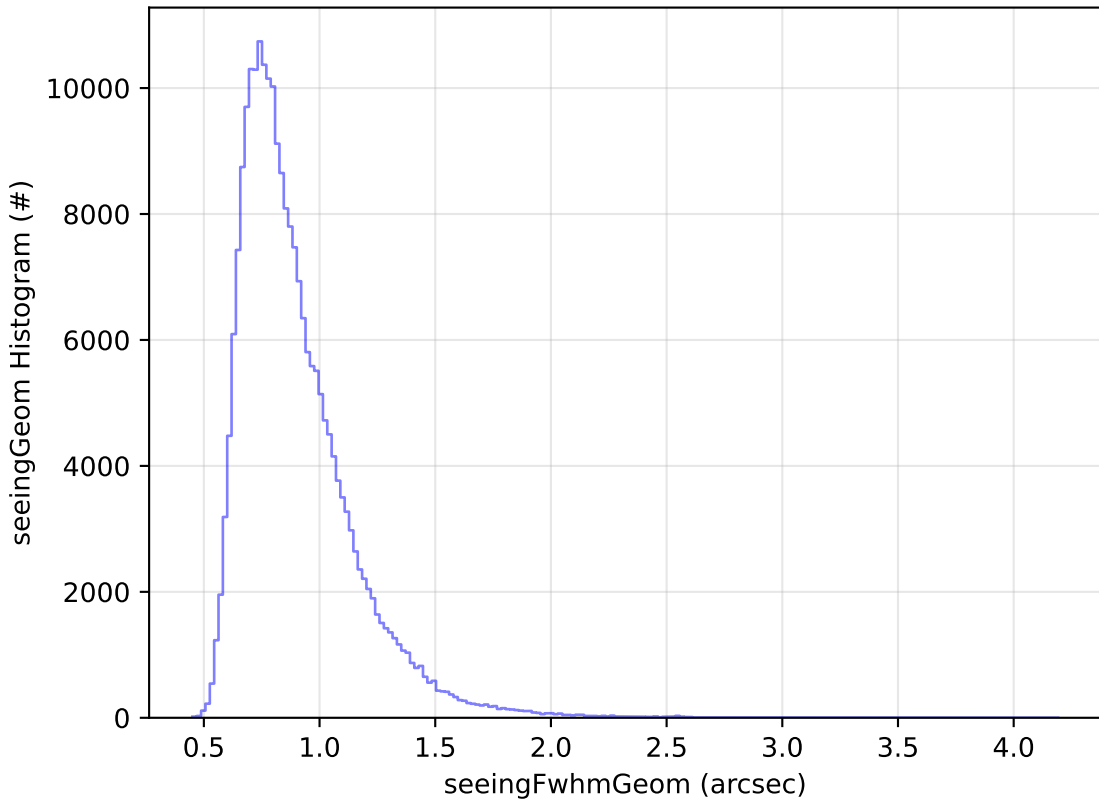
too_combined_s0.5_v3.4_10yrs Yr 1 all bands: seeingGeom Histogram
