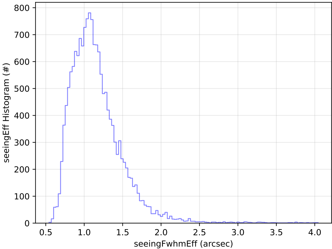
too_combined_s0.5_v3.4_10yrs Yr 1 u band: seeingEff Histogram
