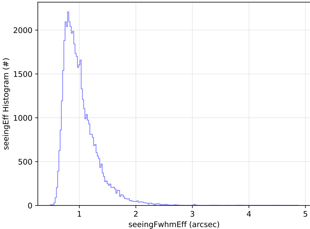
too_combined_s0.5_v3.4_10yrs Yr 1 r band: seeingEff Histogram
