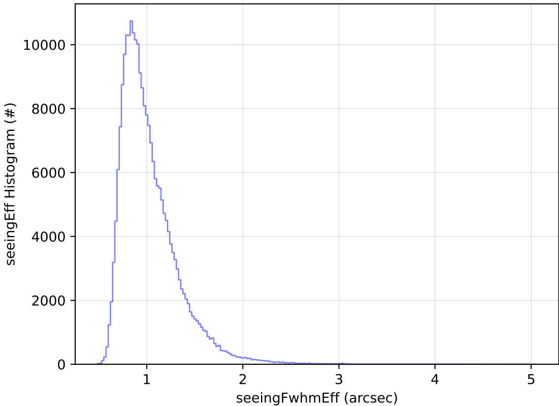
too_combined_s0.5_v3.4_10yrs Yr 1 all bands: seeingEff Histogram
