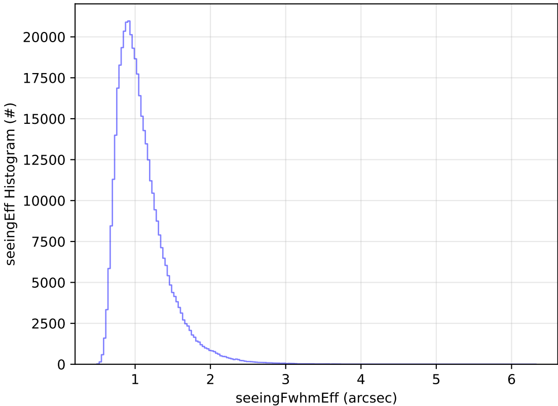
too_combined_s0.5_v3.4_10yrs WFD z band: seeingEff Histogram
