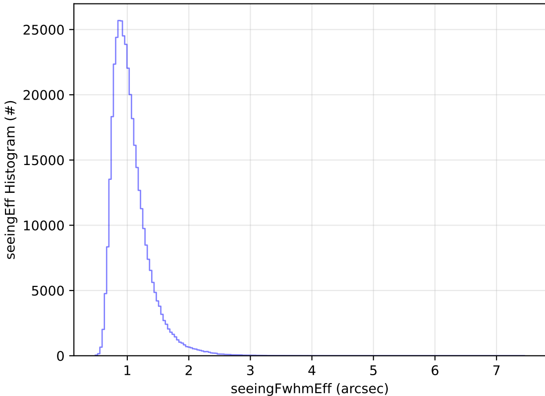
too_combined_s0.5_v3.4_10yrs WFD y band: seeingEff Histogram
