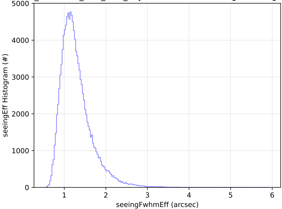
too_combined_s0.5_v3.4_10yrs WFD u band: seeingEff Histogram
