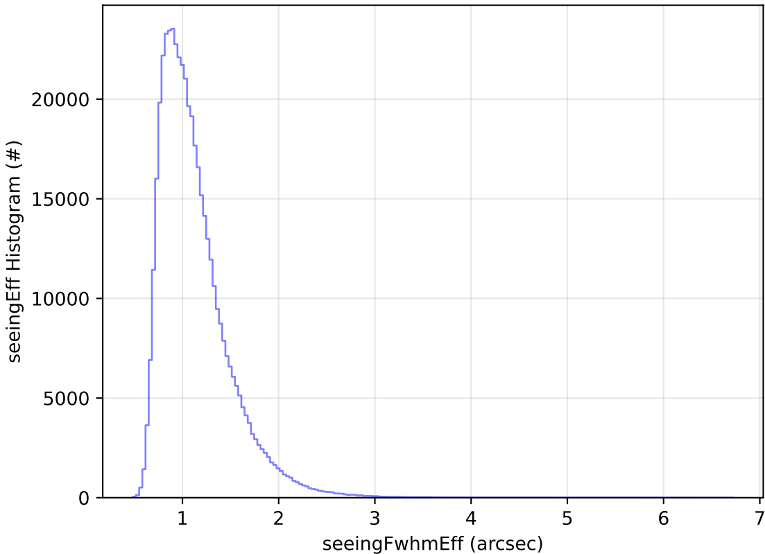
too_combined_s0.5_v3.4_10yrs WFD r band: seeingEff Histogram
