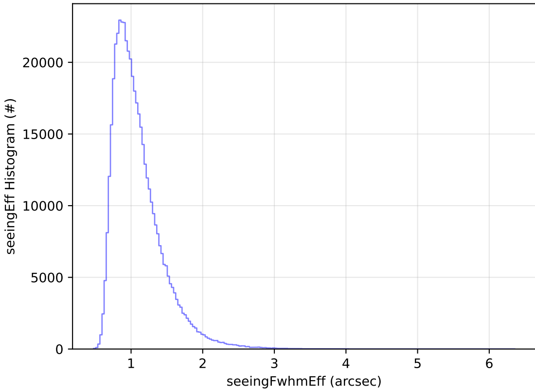
too_combined_s0.5_v3.4_10yrs WFD i band: seeingEff Histogram
