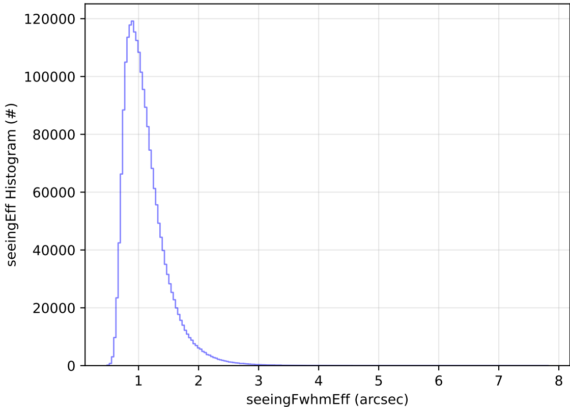
too_combined_s0.5_v3.4_10yrs WFD all bands: seeingEff Histogram
