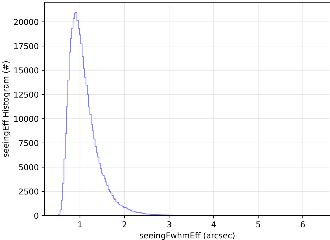
too_combined_s0.5_v3.4_10yrs All sky z band: seeingEff Histogram
