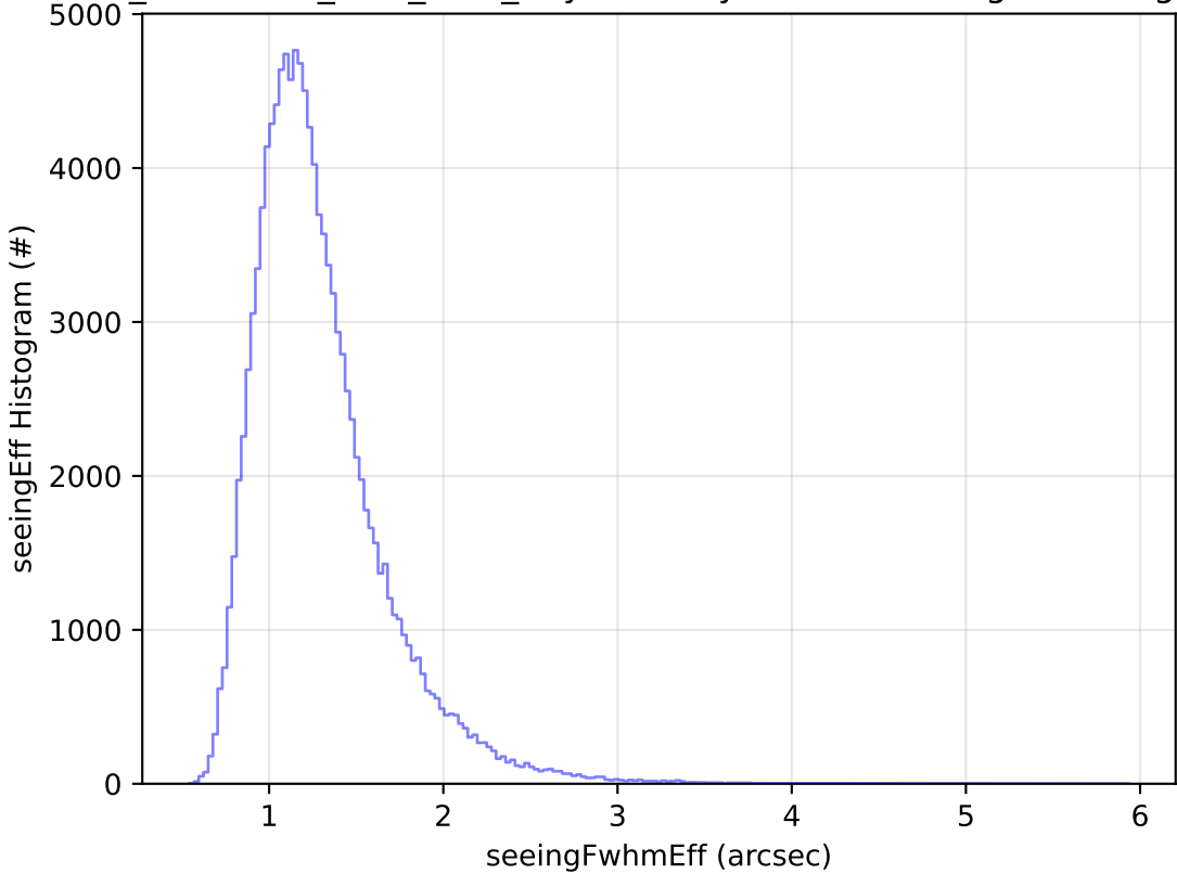
too_combined_s0.5_v3.4_10yrs All sky u band: seeingEff Histogram
