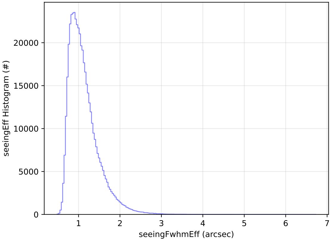
too_combined_s0.5_v3.4_10yrs All sky r band: seeingEff Histogram
