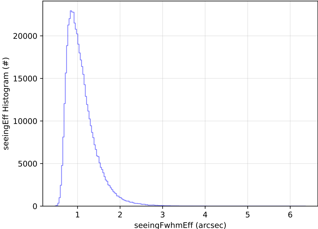
too_combined_s0.5_v3.4_10yrs All sky i band: seeingEff Histogram
