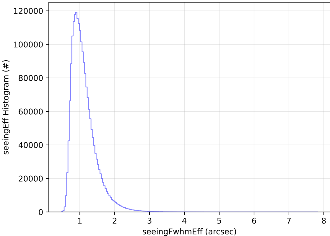
too_combined_s0.5_v3.4_10yrs All sky all bands: seeingEff Histogram
