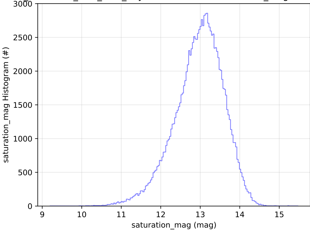
too_combined_s0.5_v3.4_10yrs WFD u band: saturation_mag Histogram
