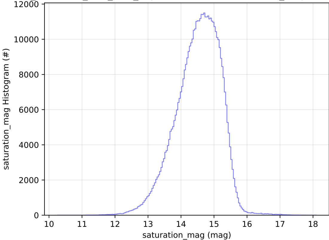
too_combined_s0.5_v3.4_10yrs WFD r band: saturation_mag Histogram
