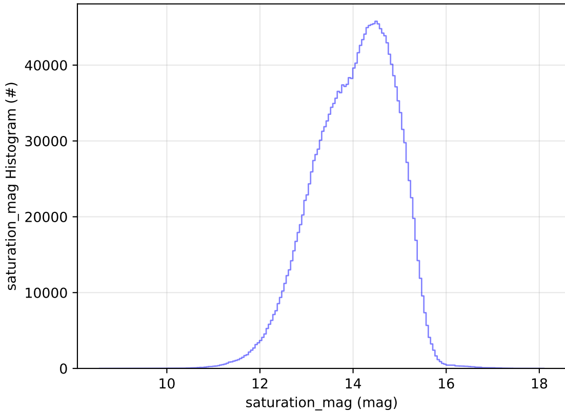
too_combined_s0.5_v3.4_10yrs WFD all bands: saturation_mag Histogram
