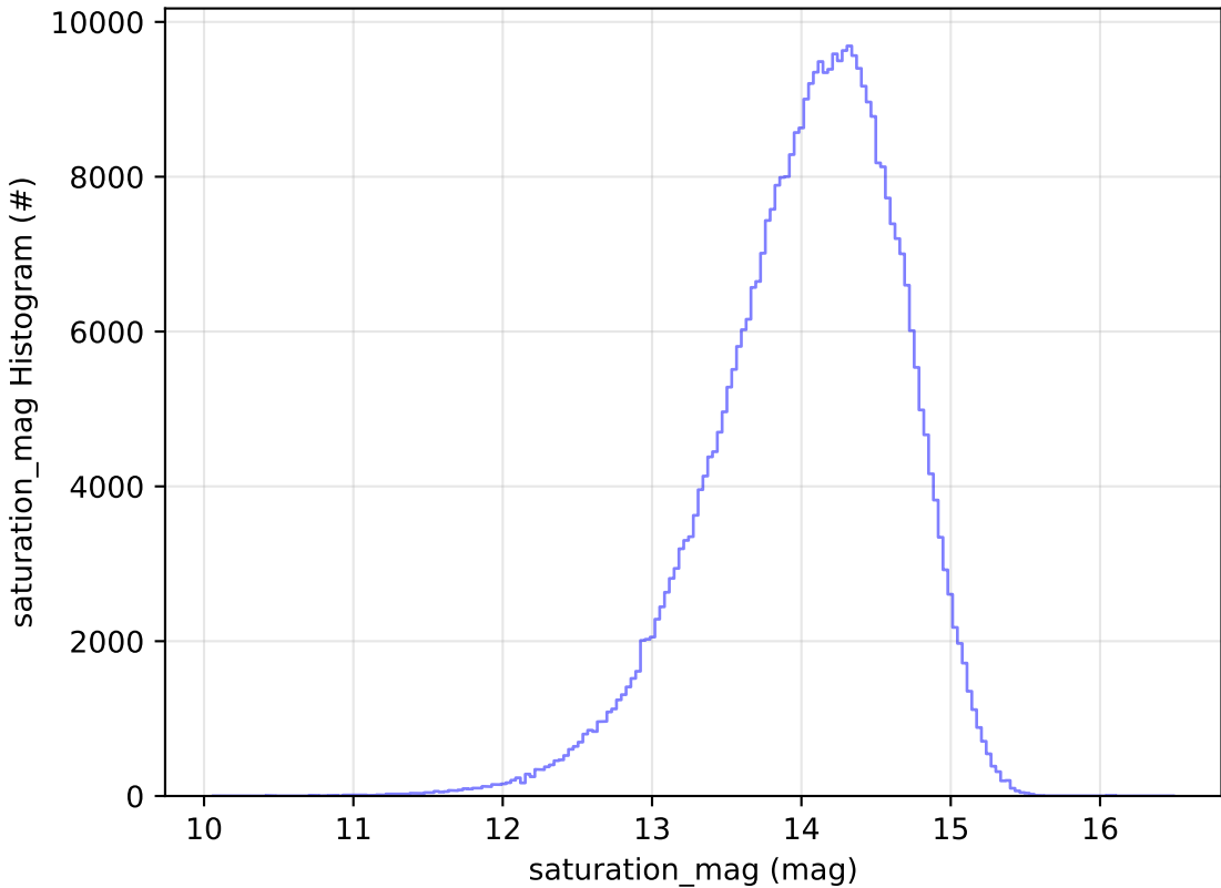
too_combined_s0.5_v3.4_10yrs All sky z band: saturation_mag Histogram
