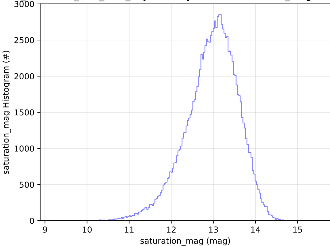
too_combined_s0.5_v3.4_10yrs All sky u band: saturation_mag Histogram
