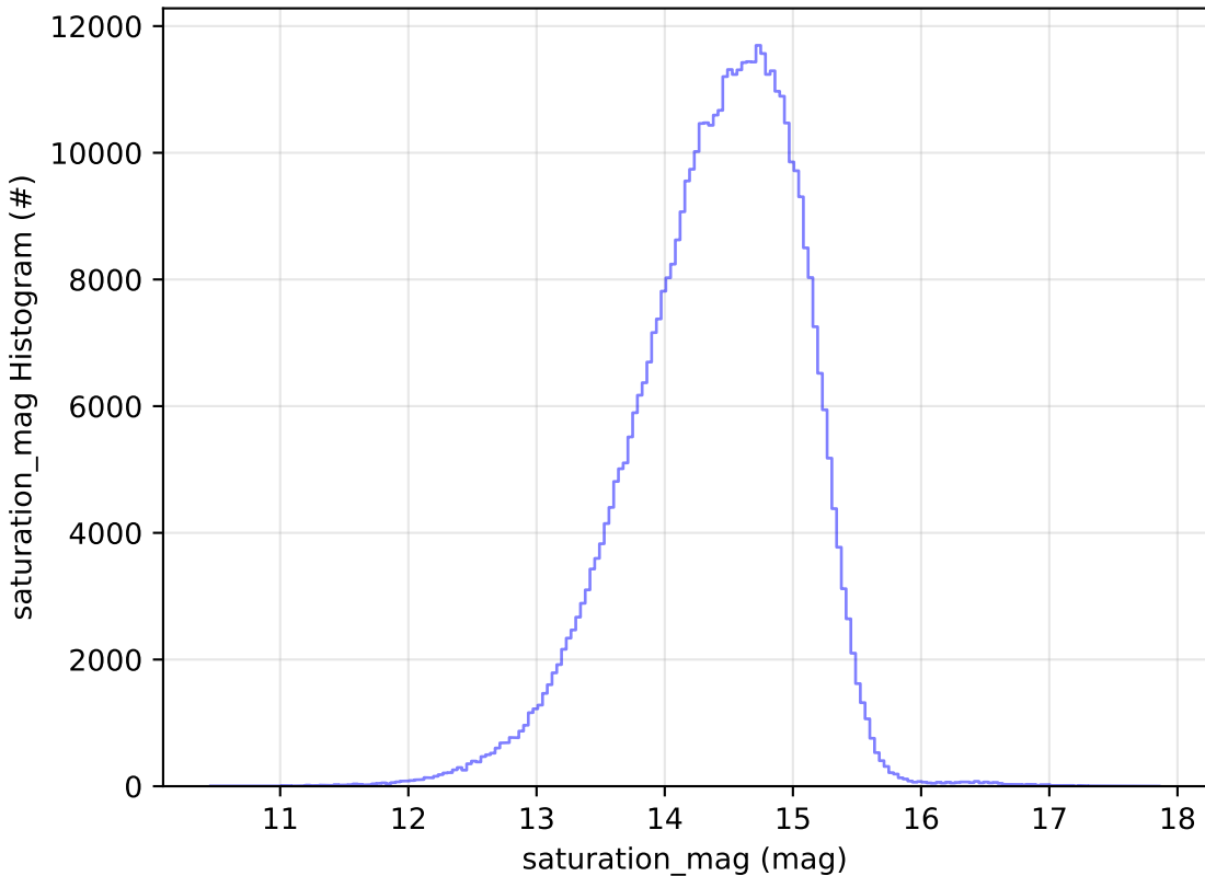
too_combined_s0.5_v3.4_10yrs All sky i band: saturation_mag Histogram
