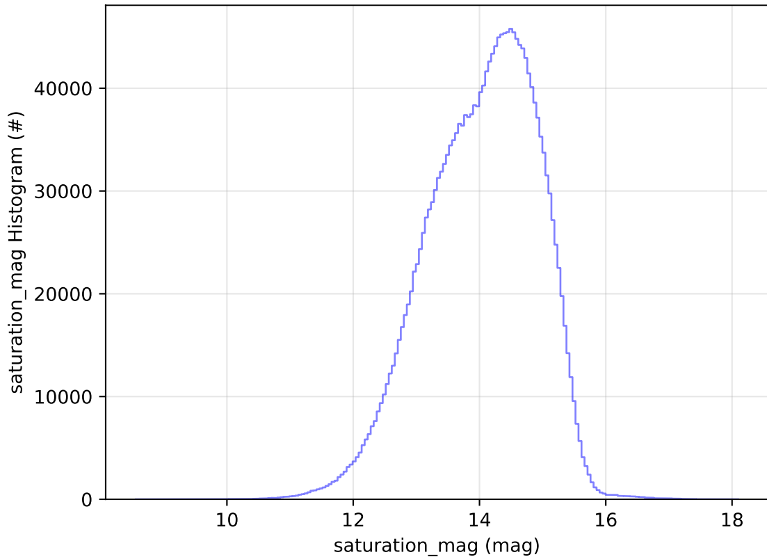
too_combined_s0.5_v3.4_10yrs All sky all bands: saturation_mag Histogram
