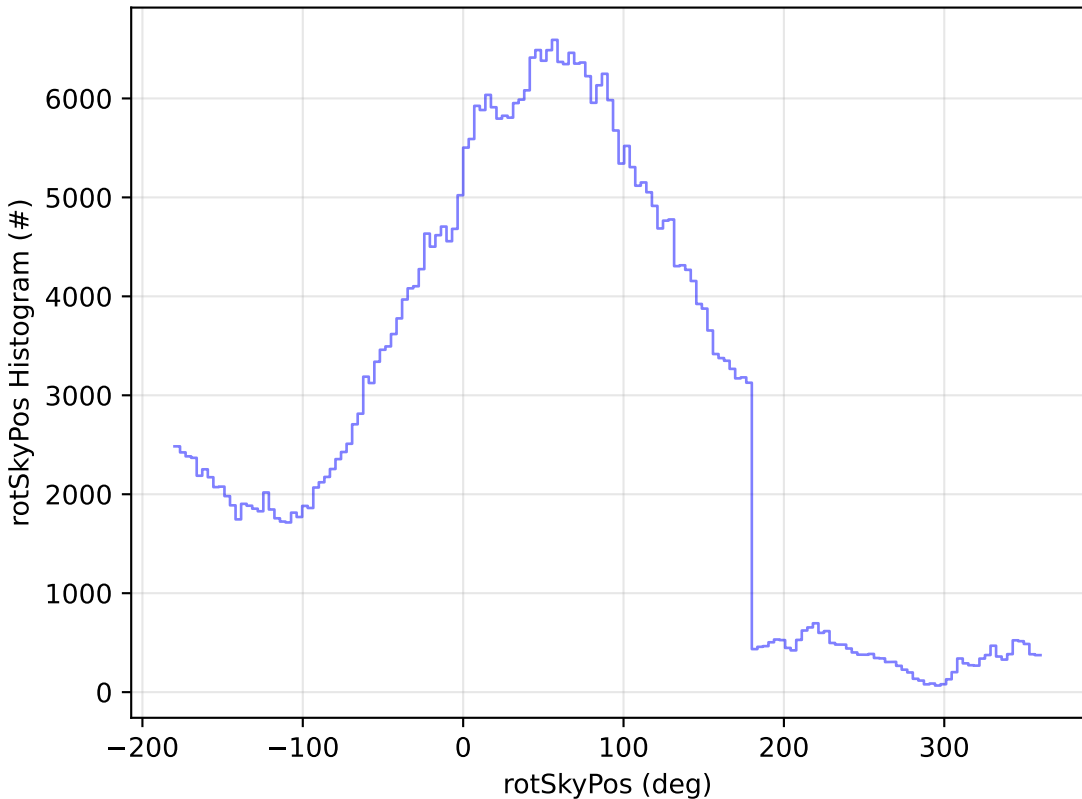
too_combined_s0.5_v3.4_10yrs WFD z band: rotSkyPos Histogram
