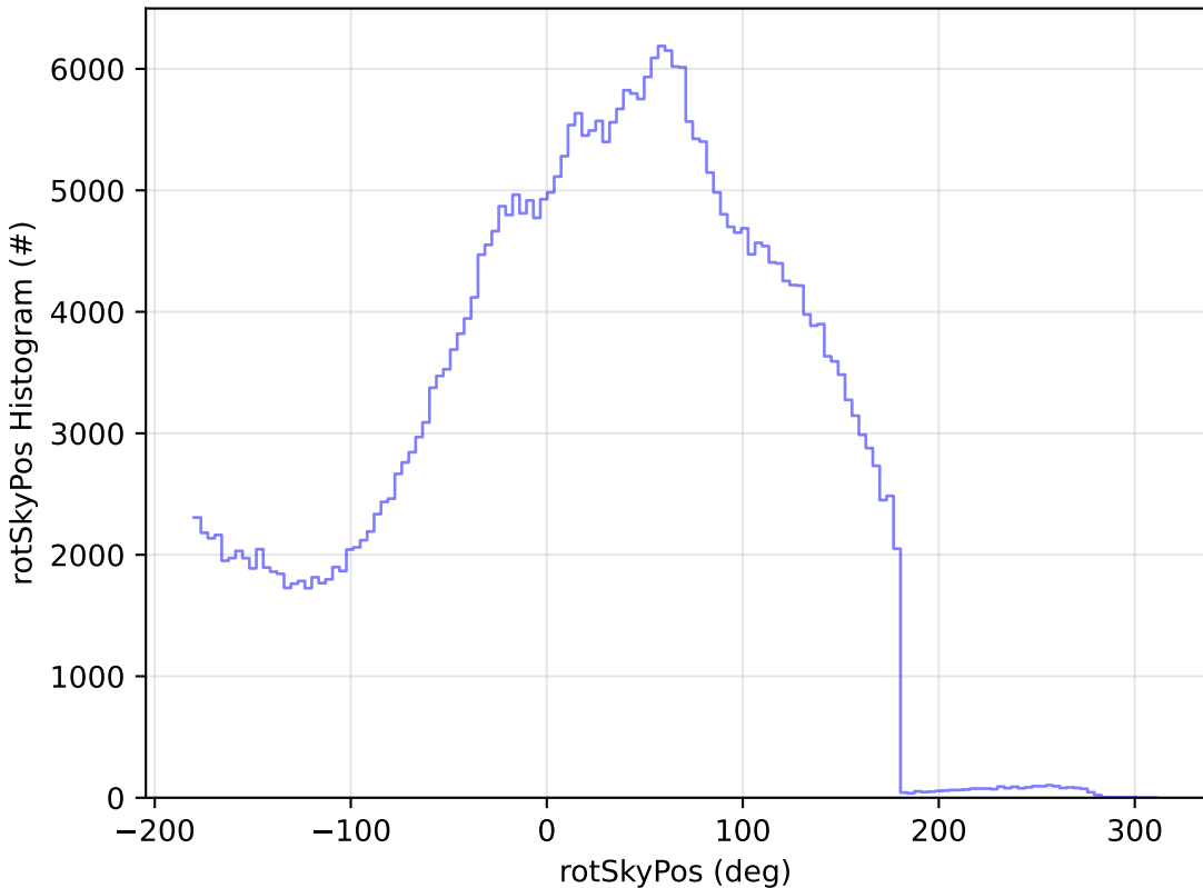
too_combined_s0.5_v3.4_10yrs WFD y band: rotSkyPos Histogram
