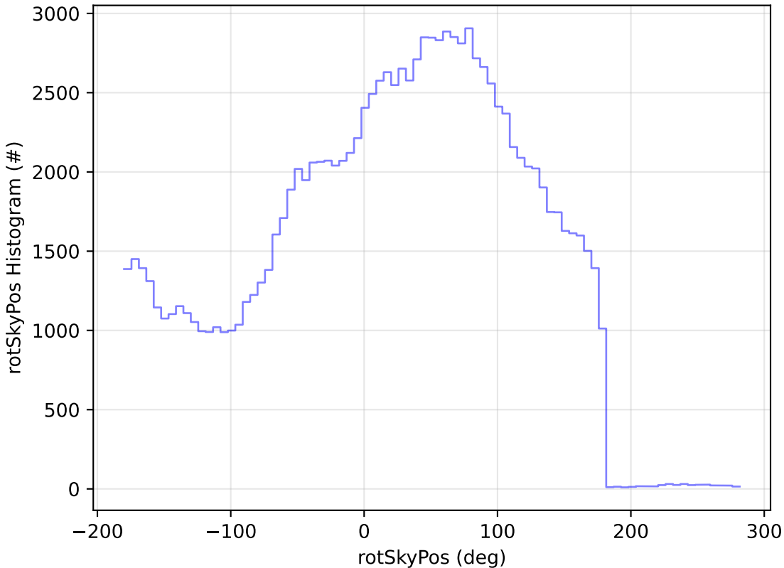
too_combined_s0.5_v3.4_10yrs_WFD_u_band: rotSkyPos Histogram
