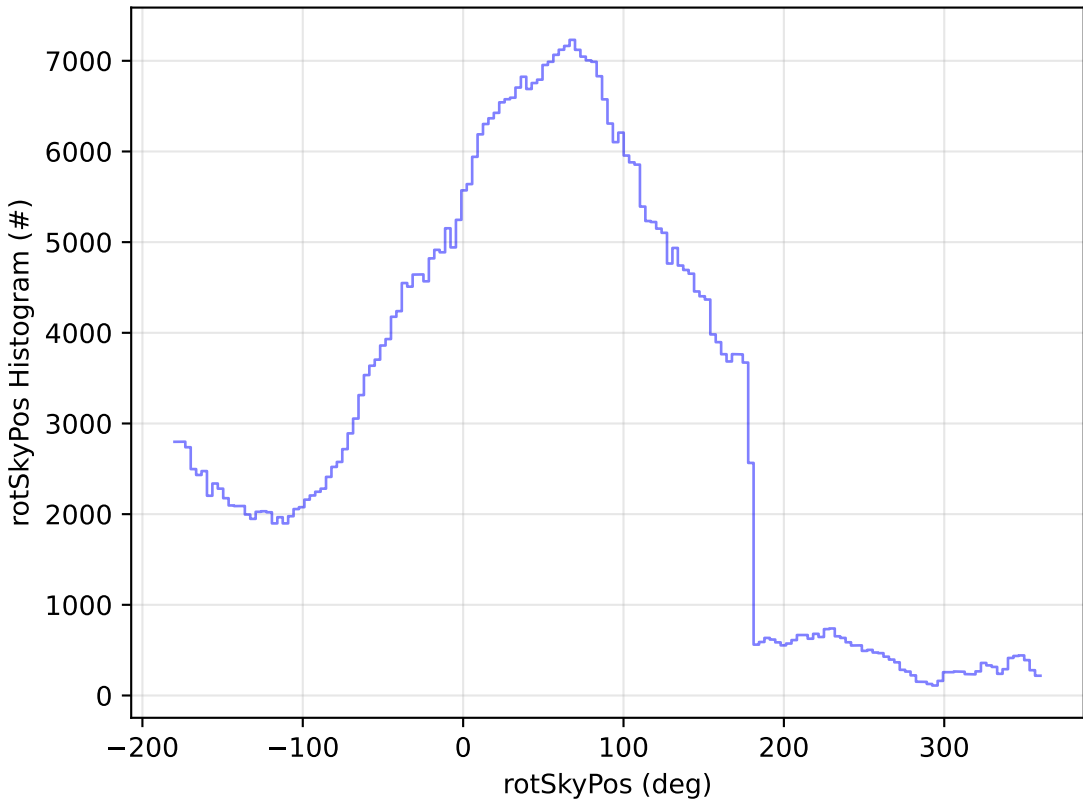
too_combined_s0.5_v3.4_10yrs WFD i band: rotSkyPos Histogram
