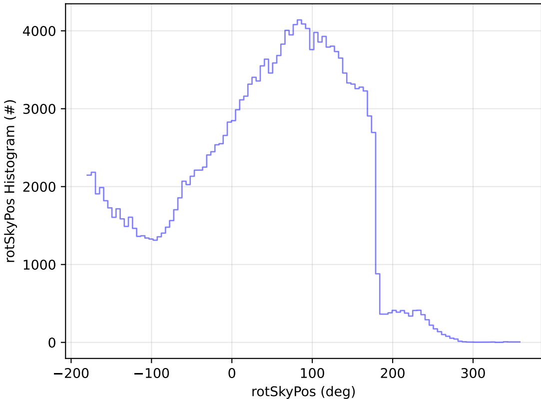
too_combined_s0.5_v3.4_10yrs WFD g band: rotSkyPos Histogram
