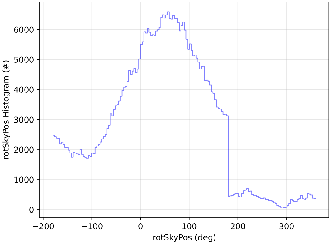
too_combined_s0.5_v3.4_10yrs All sky z band: rotSkyPos Histogram
