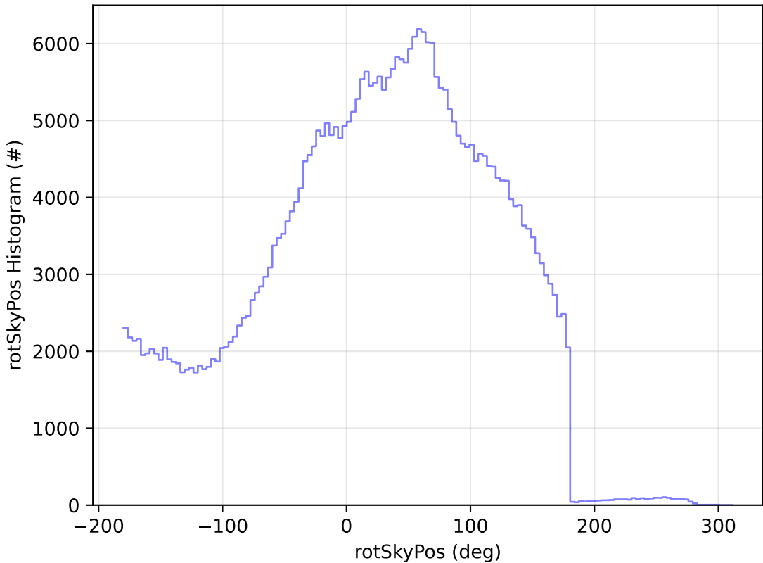
too_combined_s0.5_v3.4_10yrs All sky y band: rotSkyPos Histogram
