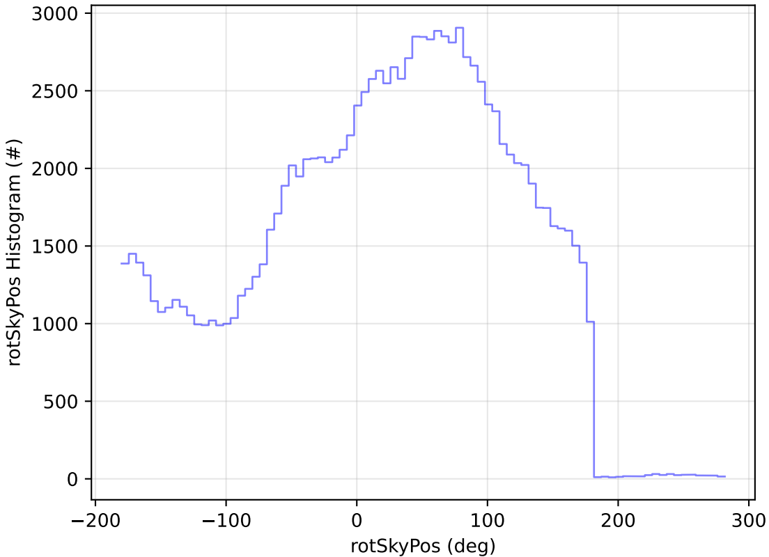
too_combined_s0.5_v3.4_10yrs All sky u band: rotSkyPos Histogram
