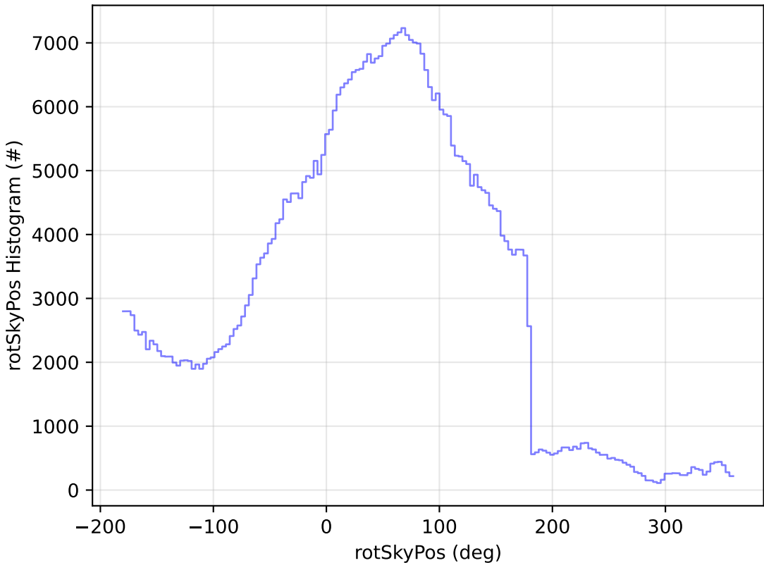
too_combined_s0.5_v3.4_10yrs All sky i band: rotSkyPos Histogram
