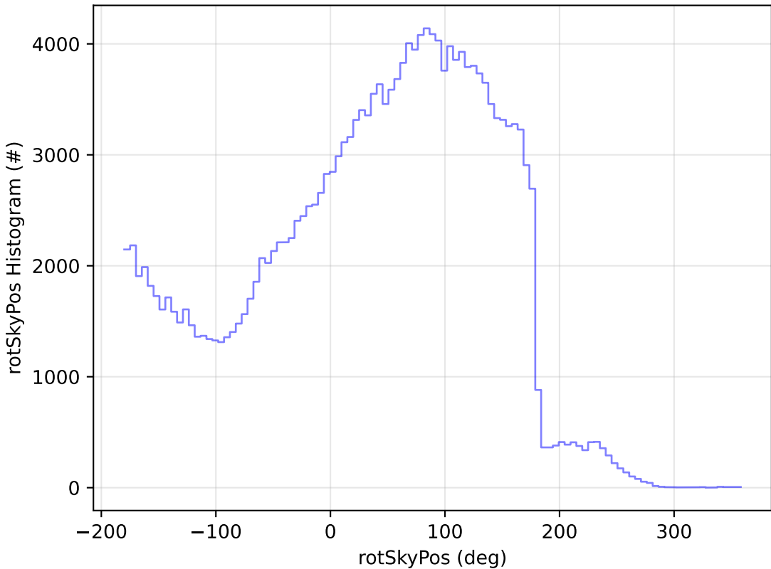
too_combined_s0.5_v3.4_10yrs All sky g band: rotSkyPos Histogram
