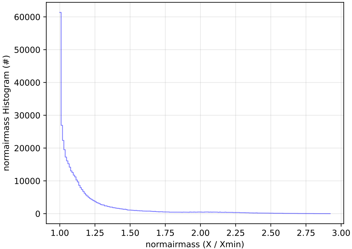
too_combined_s0.5_v3.4_10yrs WFD z band: normairmass Histogram
