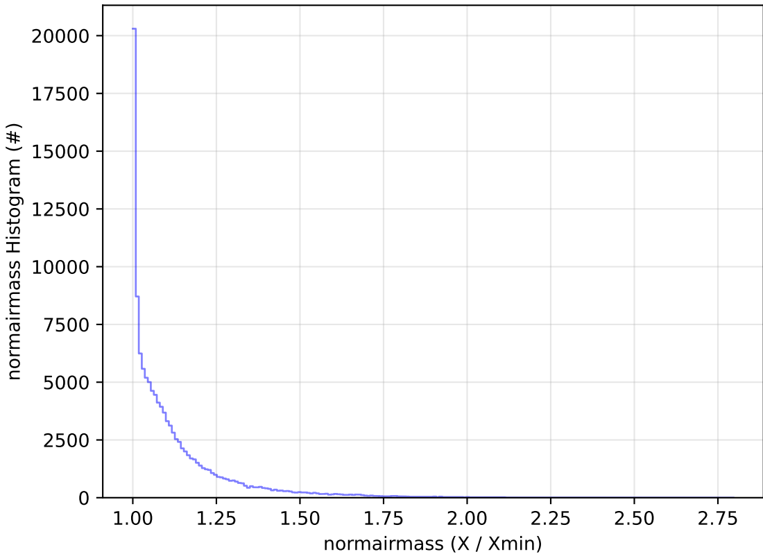
too_combined_s0.5_v3.4_10yrs WFD u band: normairmass Histogram
