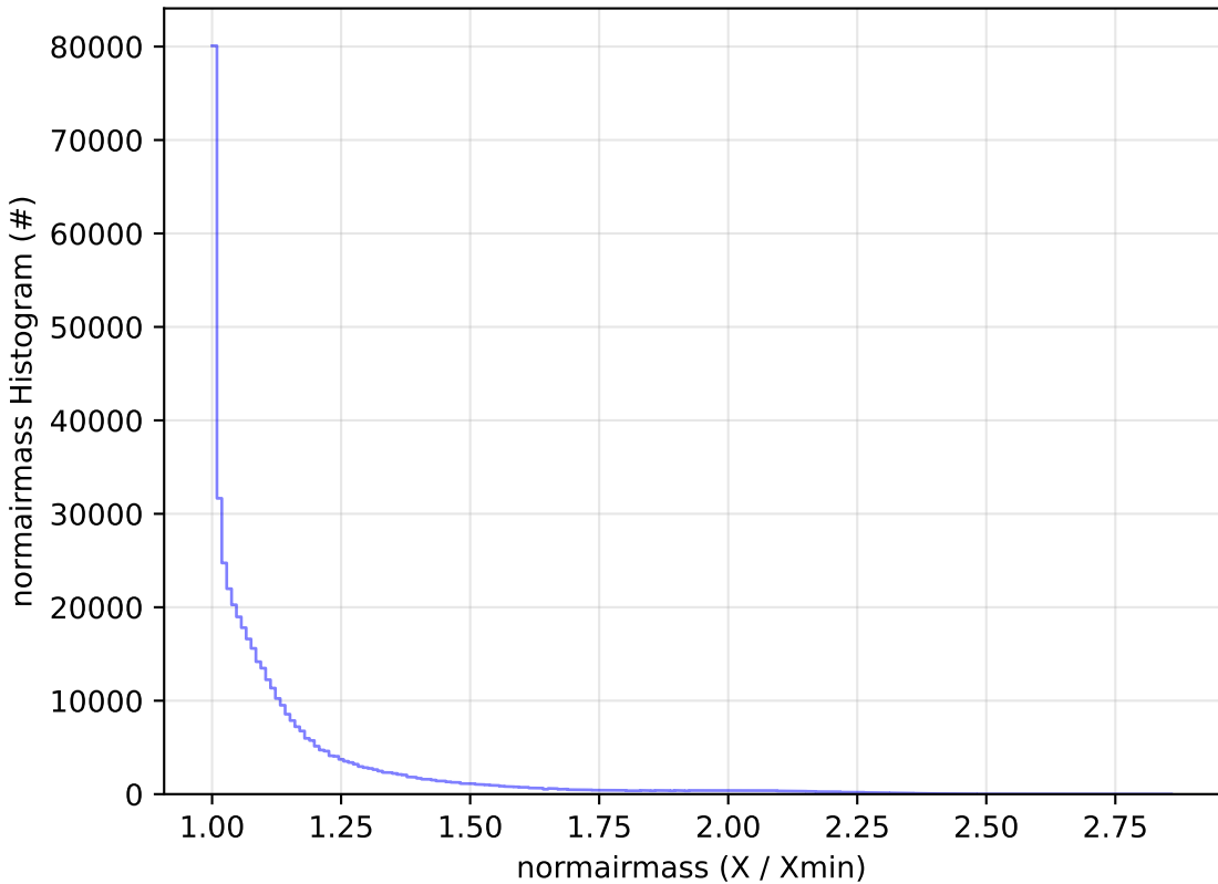
too_combined_s0.5_v3.4_10yrs WFD r band: normairmass Histogram
