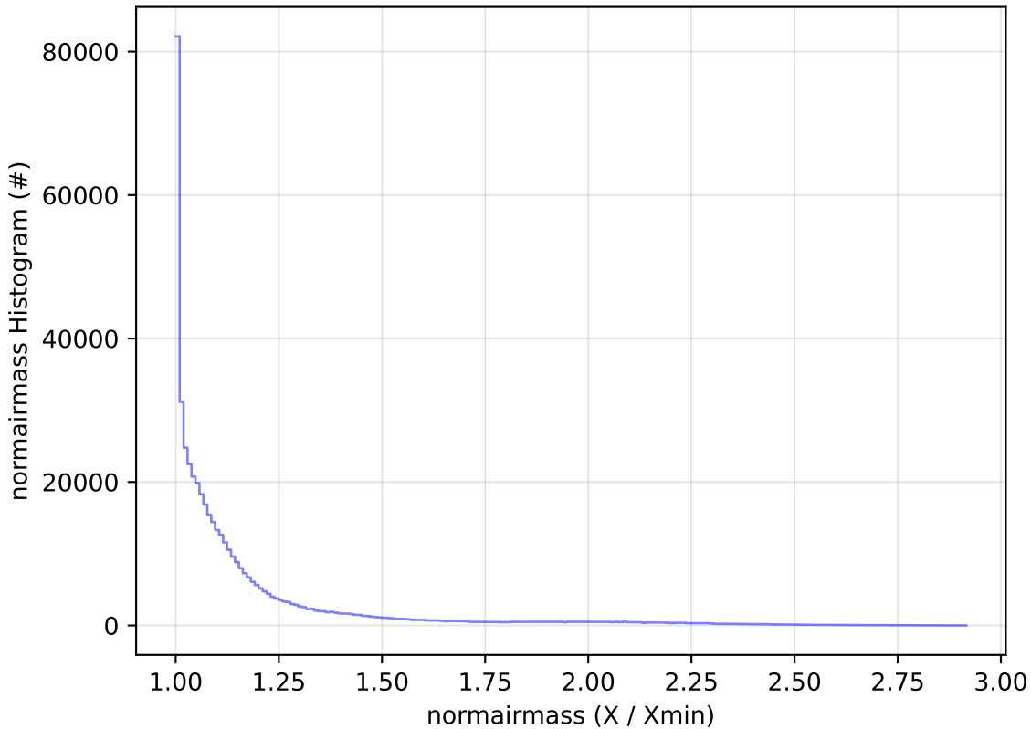
too_combined_s0.5_v3.4_10yrs WFD i band: normairmass Histogram
