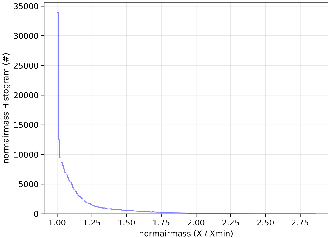
too_combined_s0.5_v3.4_10yrs WFD g band: normairmass Histogram
