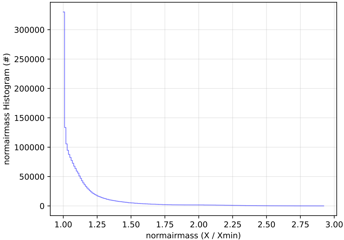
too_combined_s0.5_v3.4_10yrs WFD all bands: normairmass Histogram
