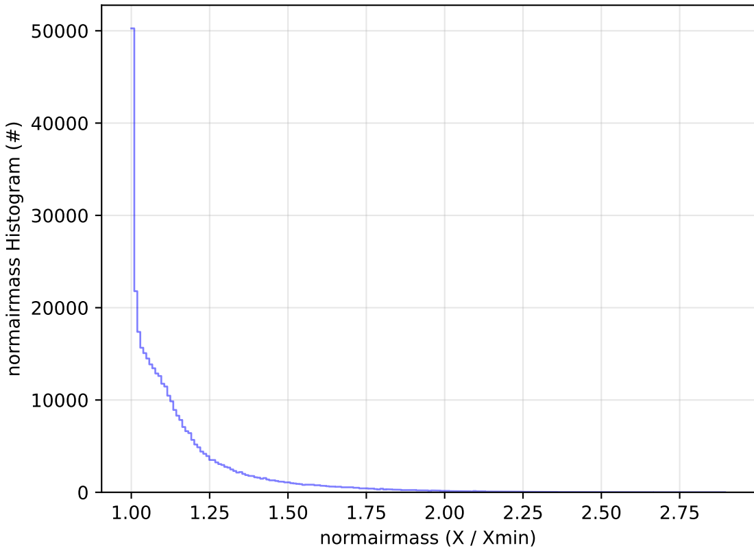
too_combined_s0.5_v3.4_10yrs All sky y band: normairmass Histogram
