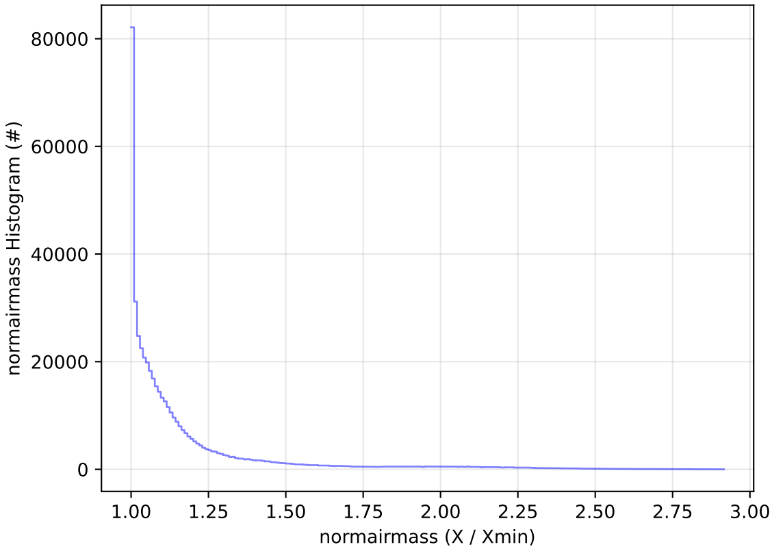
too_combined_s0.5_v3.4_10yrs All sky i band: normairmass Histogram
