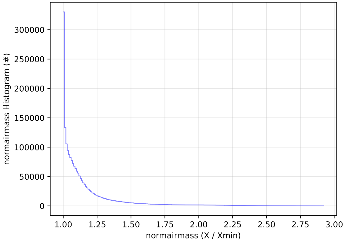
too_combined_s0.5_v3.4_10yrs All sky all bands: normairmass Histogram
