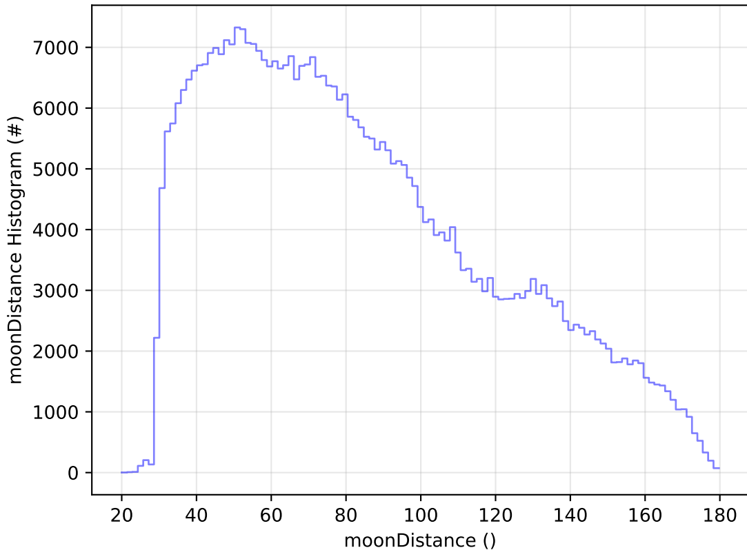
too_combined_s0.5_v3.4_10yrs WFD z band: moonDistance Histogram
