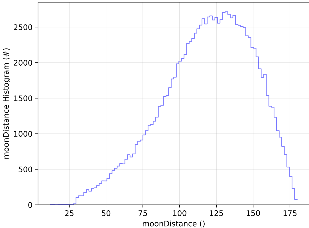
too_combined_s0.5_v3.4_10yrs WFD u band: moonDistance Histogram
